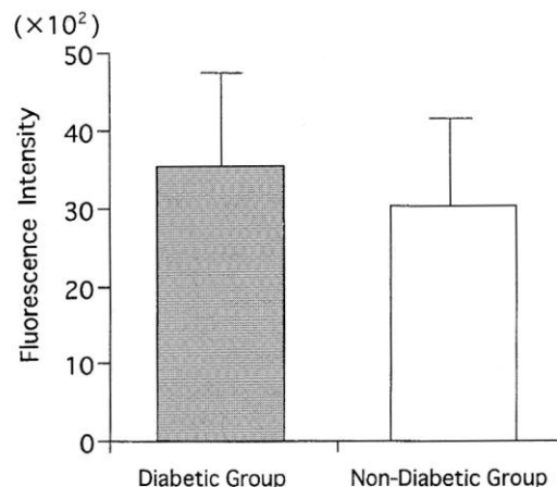
Figure 2. In vitro autofluorescence in human cataractous lenses (Ex 335 nm, Em 385 nm).
