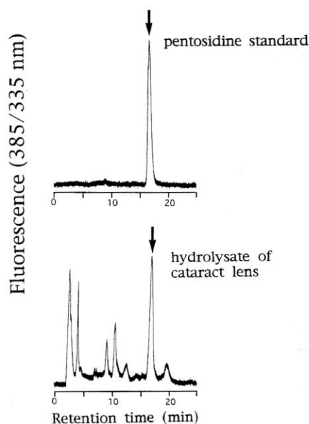
Figure 1. Chromatograms: pentosidine standard and hydrolysate of cataract lens.
