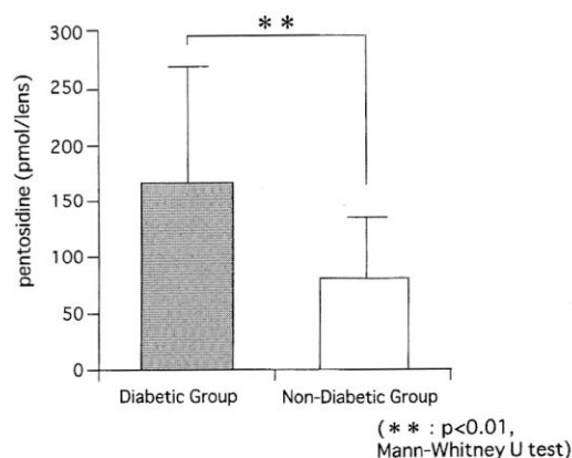
Figure 3. Amount of pentosidine in human cataractous lenses.
